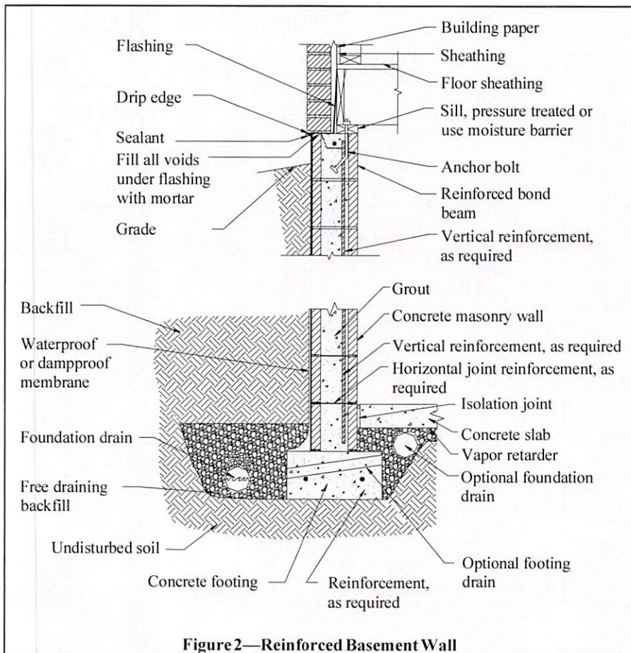
Figure 2—Reinforced Basement Wall
